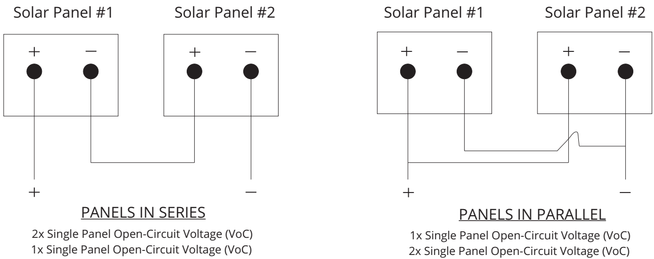
Figure 1: Schematic of two panels in series and parallel.
